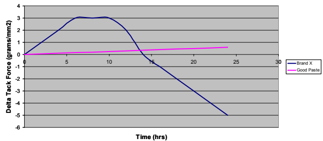
Figure 3: Comparison of tack over time of two different solder pastes. The solder paste represented by the blue line is probably not going to provide as long of a stencil life as the solder paste represented by the pink line.
