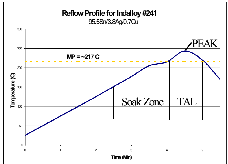
Figure 5: This is a graphical representation of a typical Pb-free reflow profile. The three critical aspects of the profile (soak zone, time above liquidus, and peak temperature) are identified.
