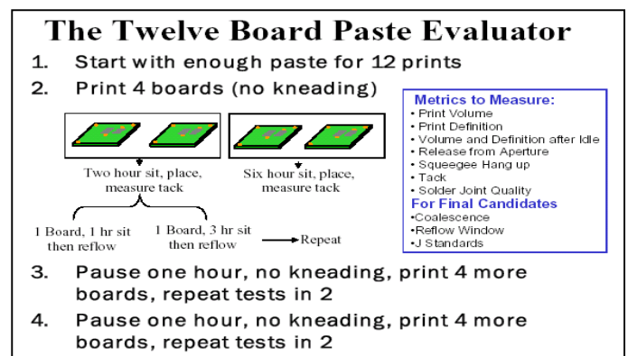
Figure 7: Stencil printing technique for evaluating the stencil life and response to pause of solder pastes.
