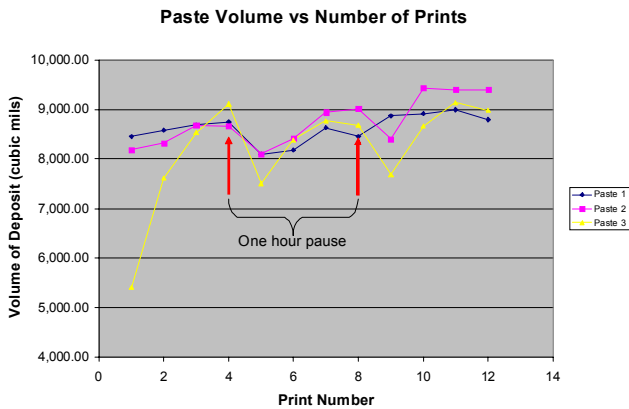
Figure 4: Comparison of print volumes between solder pastes with dramatically different “response to pause.” Paste #3 is clearly inferior with respect to this test.
