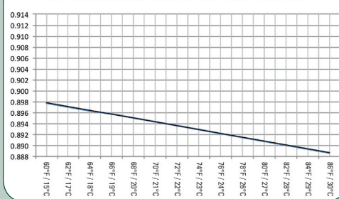
WF-1098 SPECIFIC GRAVITY VS. TEMPERATURE
