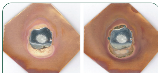
CW-232 SAC305 0 Hours
