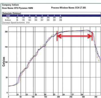
Peak Temp: 205°C Time @ Peak 90–100 seconds
