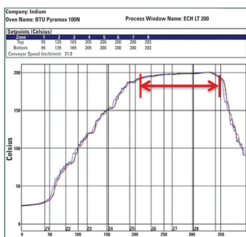
Peak Temp: 200°C Time @ Peak 120–140 seconds
