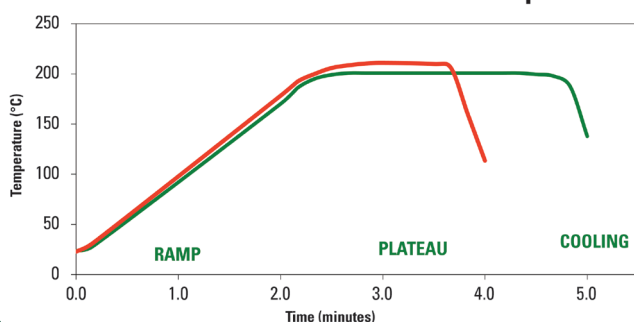
Durafuse® LT Reflow Profile Examples
