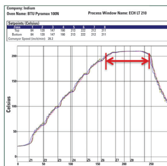
Peak Temp: 210°C Time @ Peak 60–70 seconds
