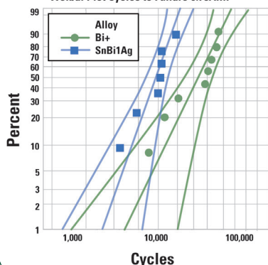
LED Cycling: Bi + vs. SnBi1Ag Weibull Plot Cycles to Failure 0.75AMP
