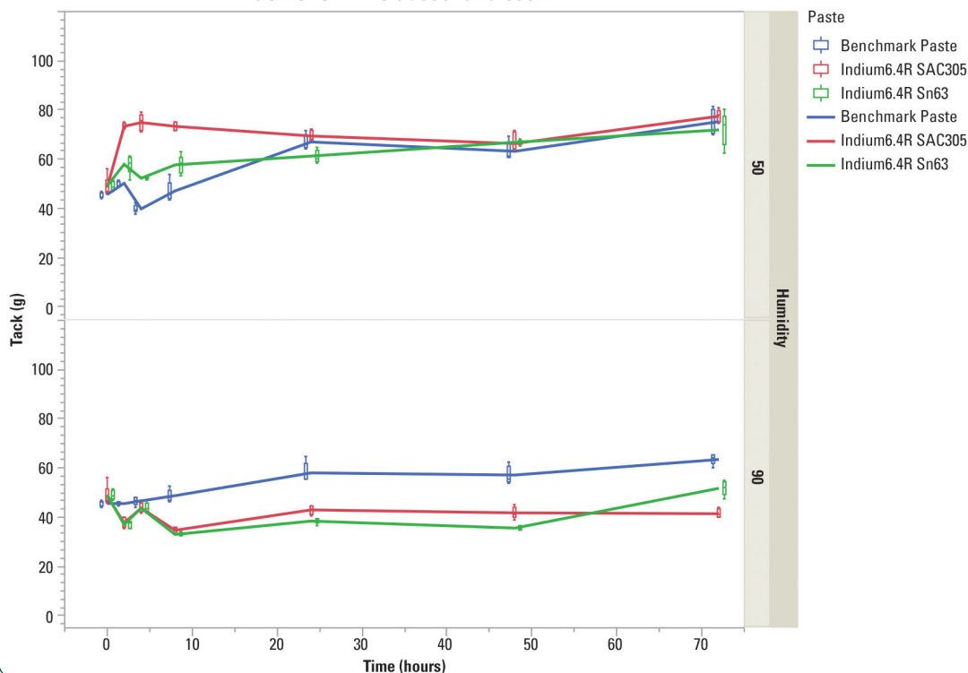
Tack Over Time at 50% and 90% RH
