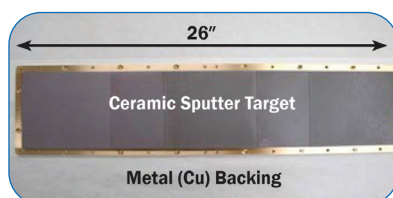
Ceramic target bonded to copper backing plate.
