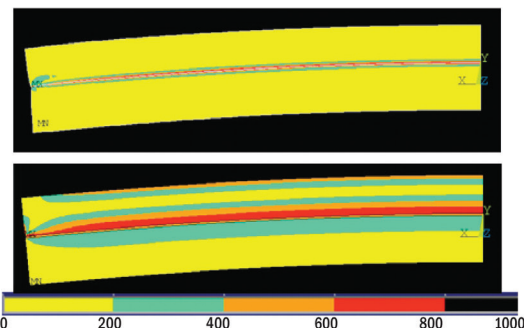
FEA modeling of conventional and NanoBond® joints. The strain energy of the NanoBond® joint is 1/8 that of the conventional bond and deflection is an order of magnitude less.
