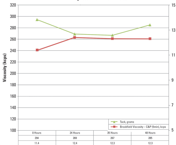
Viscosity and Tack Over Time
