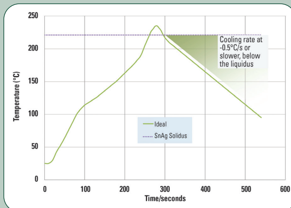
Profile optimized for thin die/thin substrate flip-chip.
