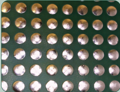
Hole fill test board.
