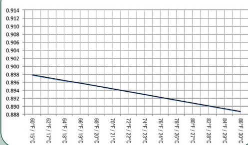
WF-1098 SPECIFIC GRAVITY VS. TEMPERATURE
