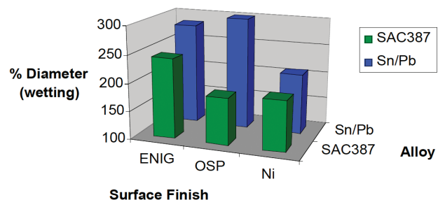
Solder Wetting Test
